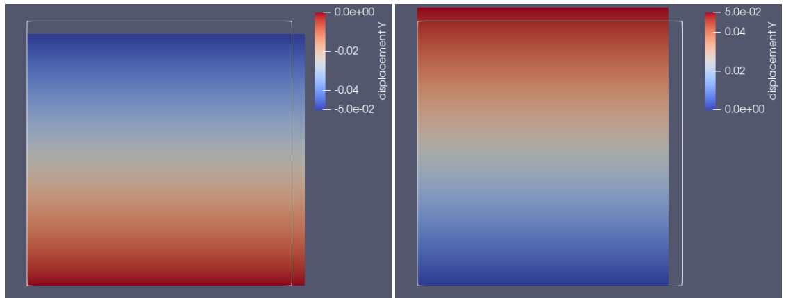
Figure 6: Biaxial test results for different BCs: shown are the mixed cases from Table 3.
