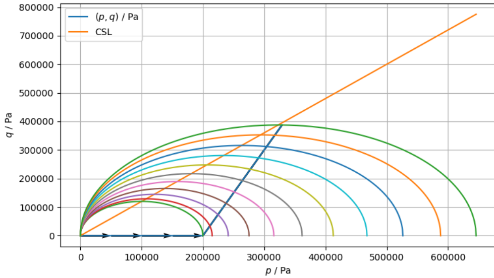
Figure 9: Triaxial benchmark results: depicted is the stress trajectory and the evolving yield surfaces as well as the CSL.
